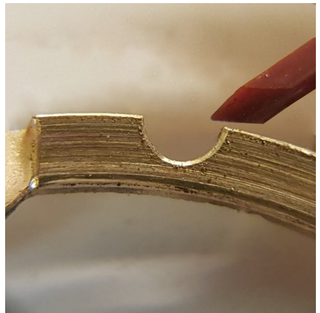
New GoS chapter ring in Bronze – Fine degaussite stone is used to shape the bevels before polishing
