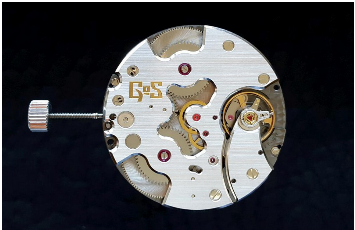
GoS02 – Technotime TT718
